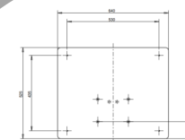
BASE FOR COLUMN Can be fixed on floor Cod: 07182
