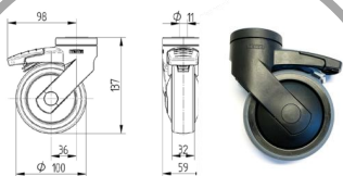
CASTOR100 Kit 4 wheels cod: 04488
