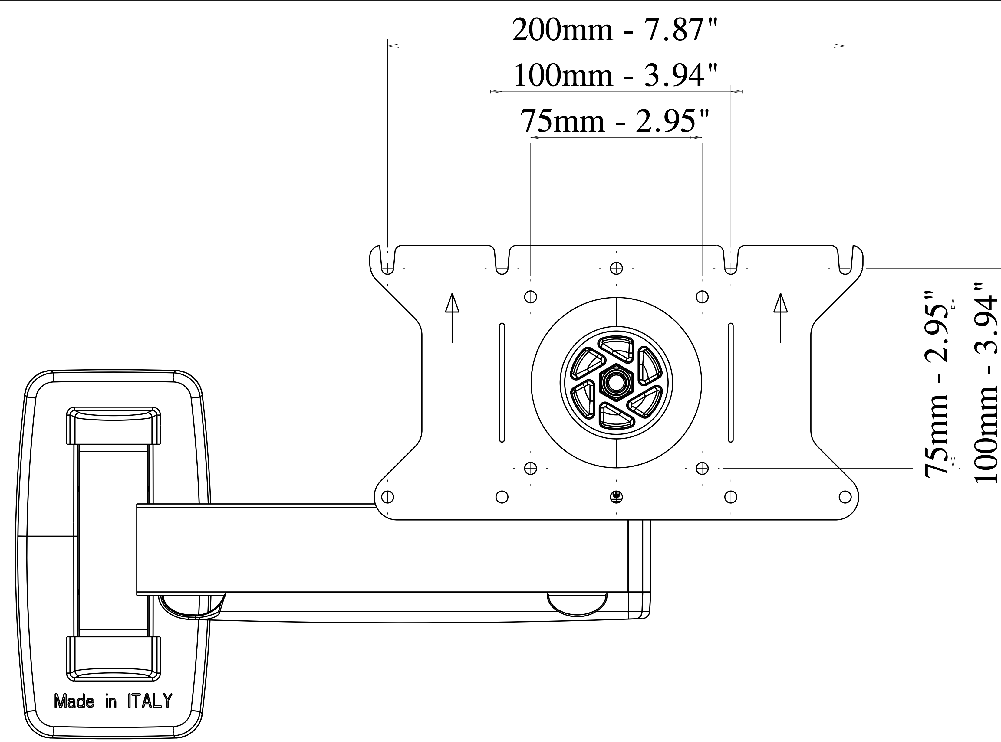
VISTA FRONTALE - FRONT VIEW
