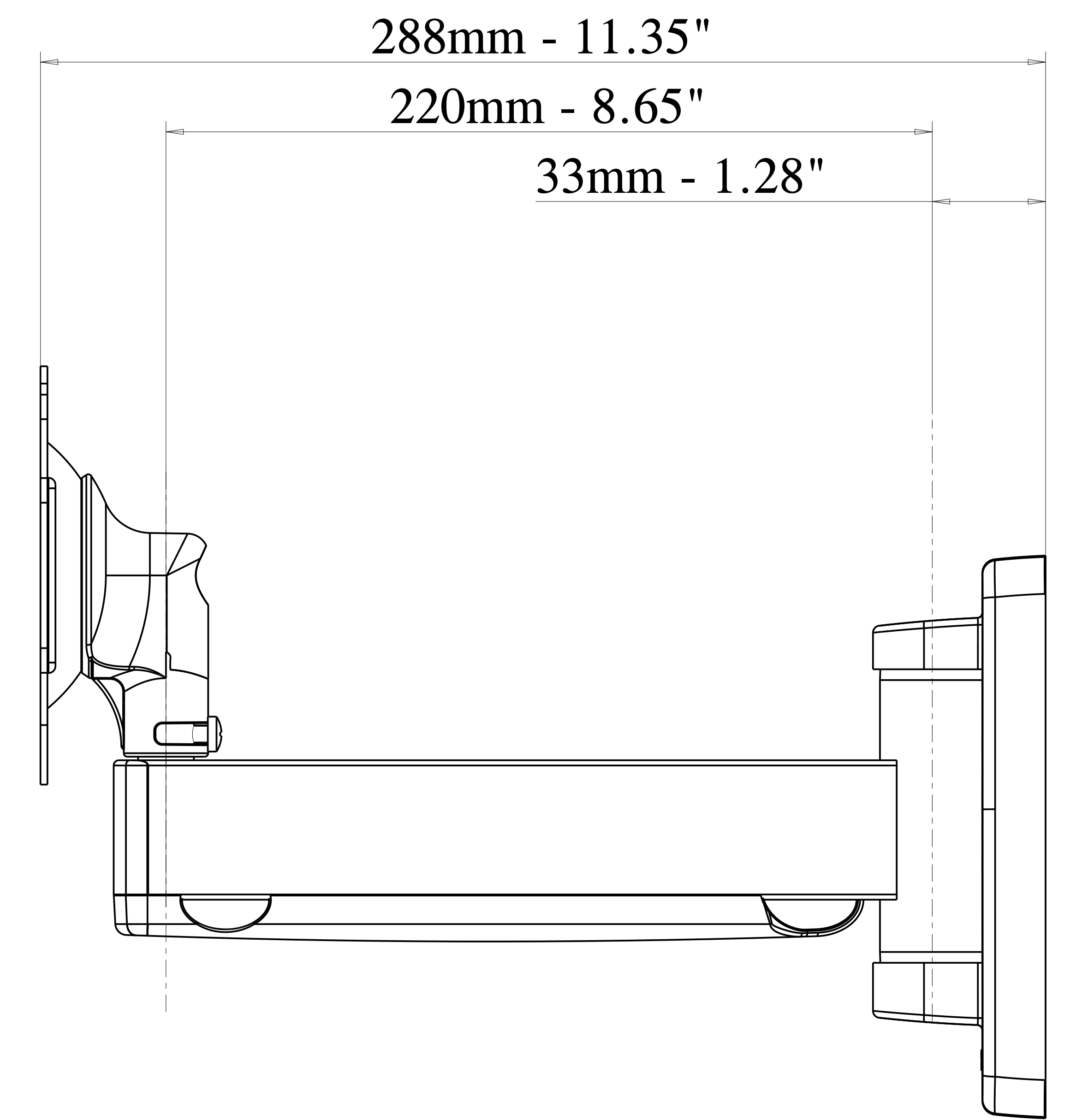
VISTA LATERALE - SIDE VIEW
