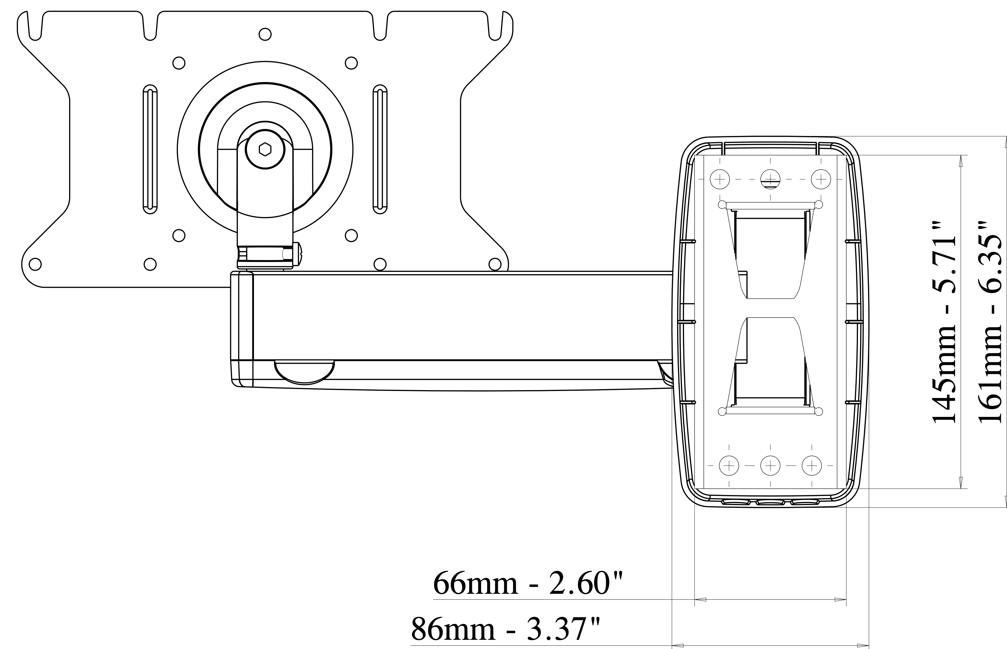
VISTA DIETRO - REAR VIEW
