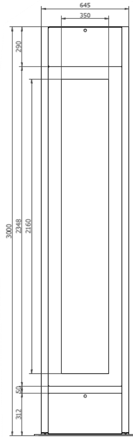
TOTEM ESSENTIAL FOR ULTRA STRETCH DISPLAY (like LG 86BH5F-M)
